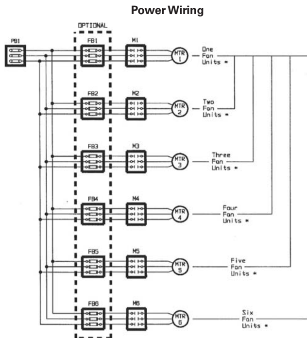
Figure 4: Single Fan-Width Units
