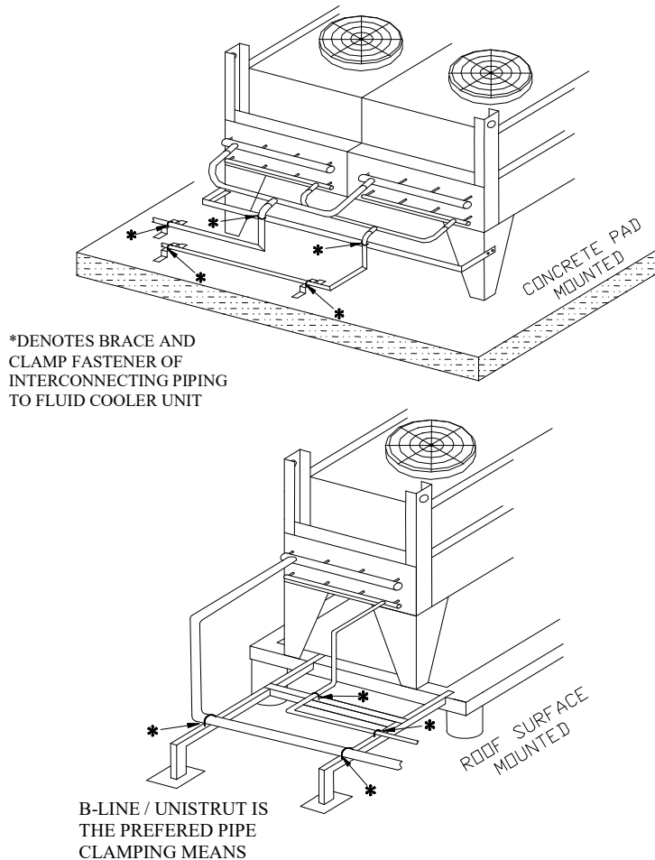
FIGURE 8 UNIT MOUNTING AND PIPING
