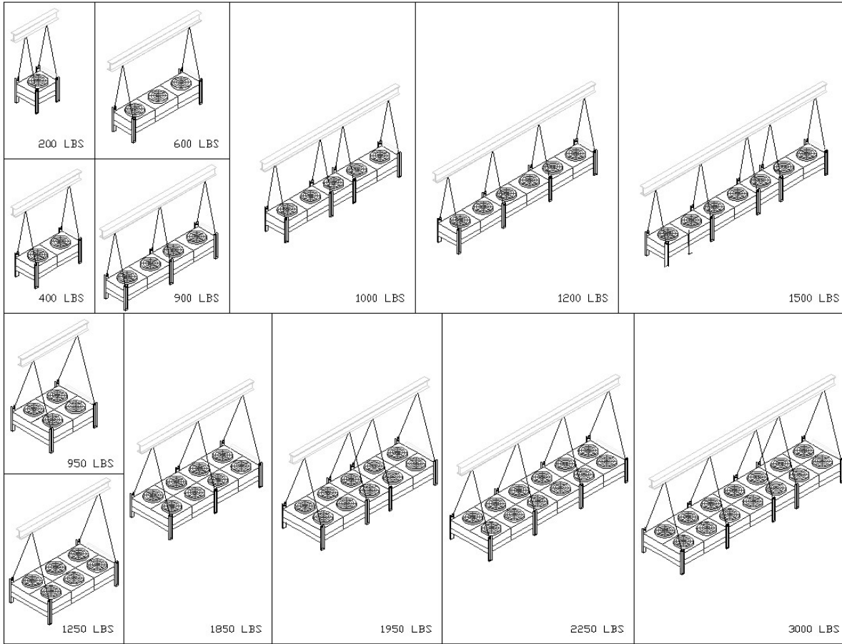
FIGURE 5 RIGGING AND LIFTING FOR 24" FAN UNITS
