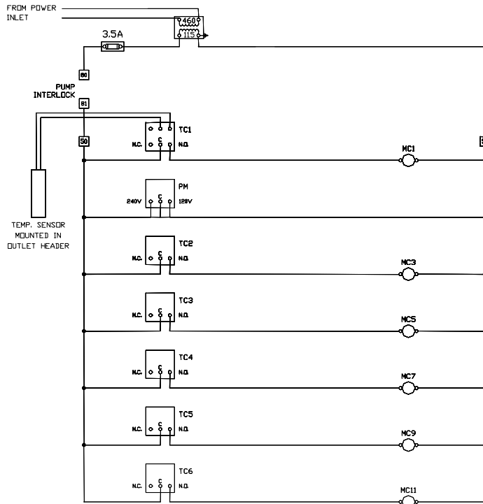
FIGURE 13 CONTROL PANEL WIRING DIAGRAMS
