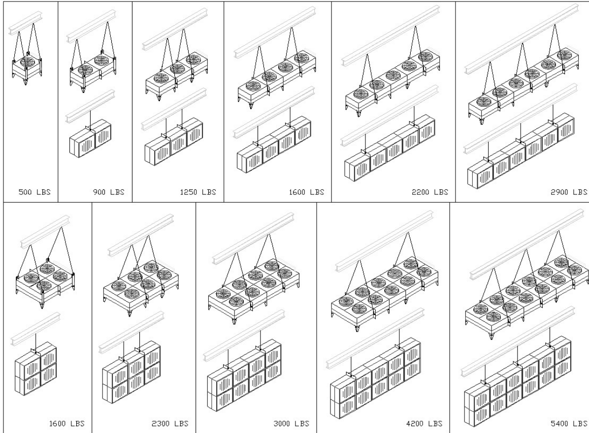
FIGURE 4 RIGGING AND LIFTING FOR 30" FAN UNITS
