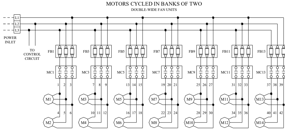
FIGURE 13 CONTROL PANEL WIRING DIAGRAMS
