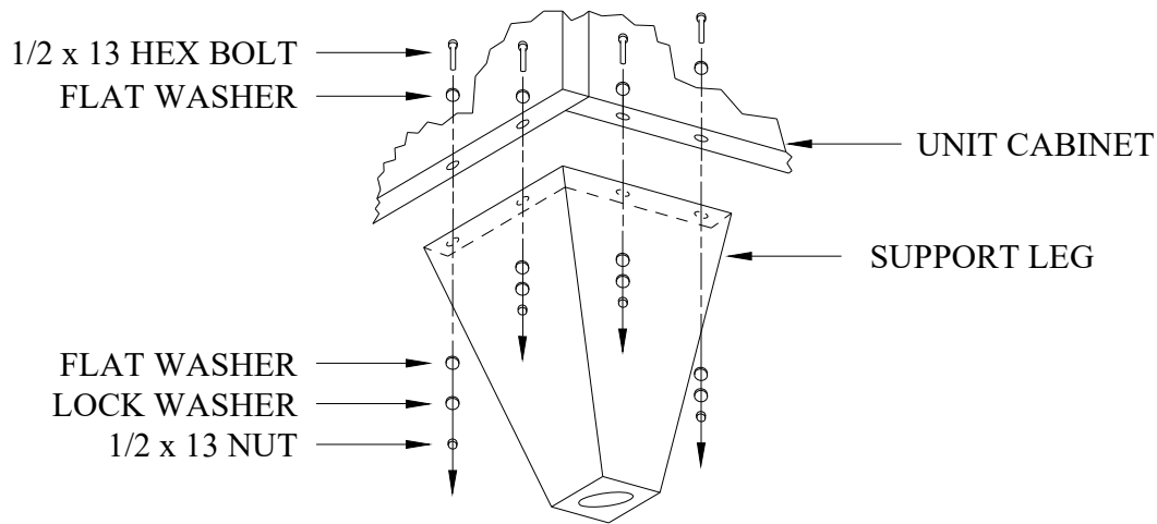
FIGURE 6 STANDARD 22" & 42" LEG ASSEMBLY
