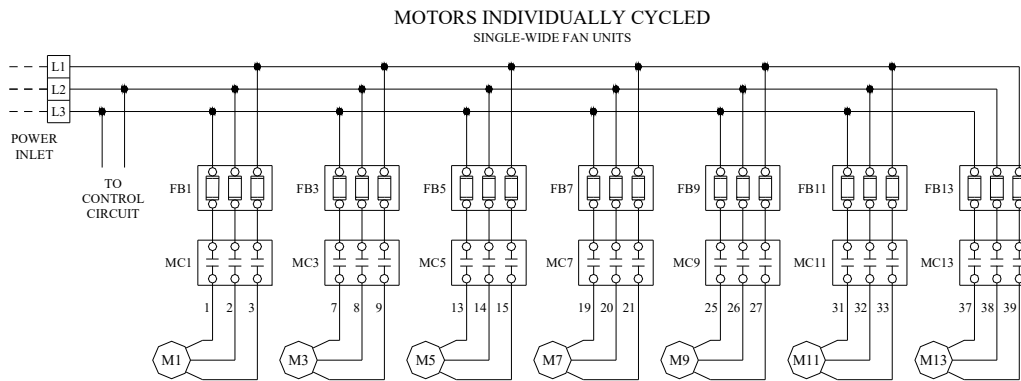
FIGURE 11 FAN CYCLING WIRING DIAGRAMS (-311)
