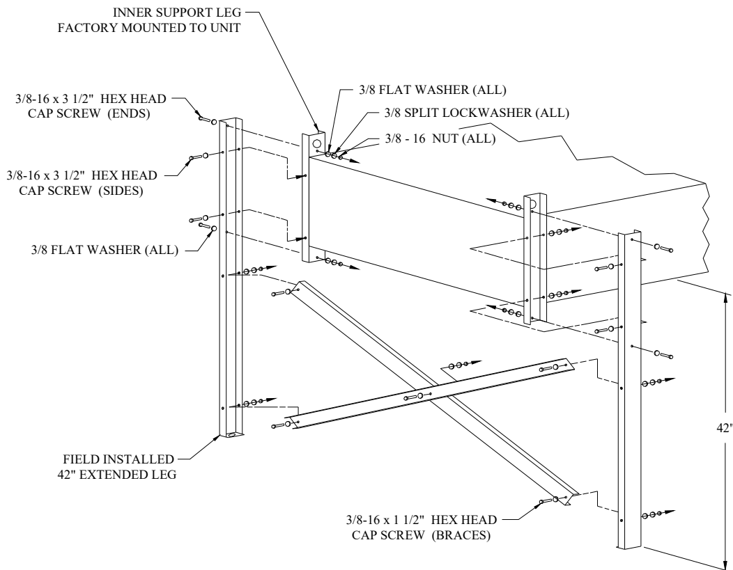
FIGURE 7 STANDARD 42" LEG & BRACING ASSEMBLY
