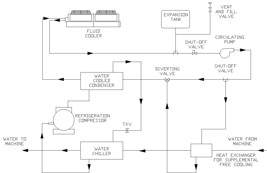
FIGURE 9 TYPICAL PIPING
